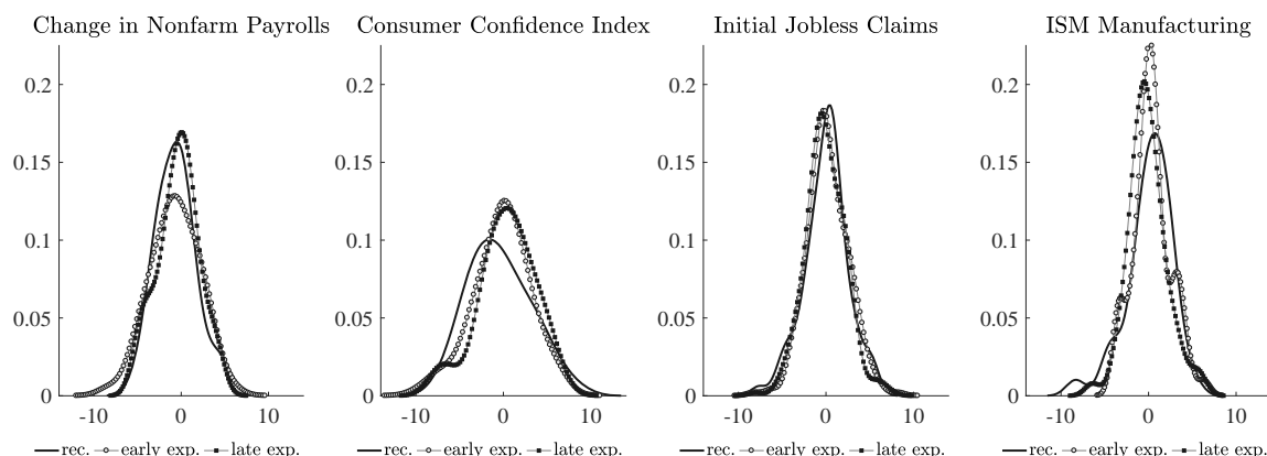
Figure E.5: Distribution of the MNA Surprises
